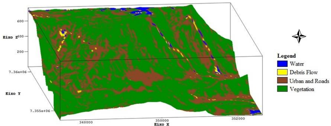
Figure 6. Debris flow perspective vision for SVM/NDVI classification and the digital terrain model overlay.
