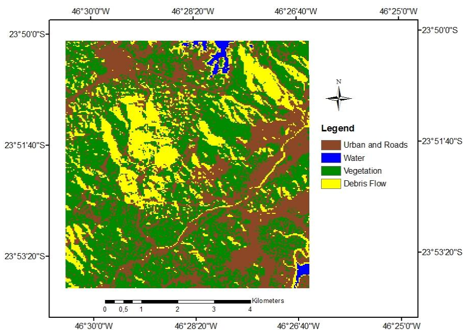
Figure 2. MLC based on 2000 Landsat image for the study area.
