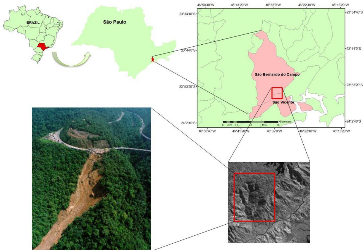
Figure 1. Study area location and debris flow picture. Adapted from Ogura (2009).
