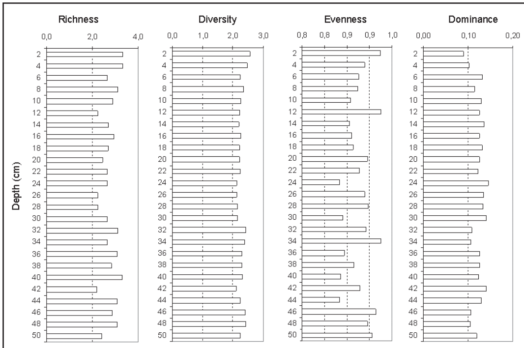
Figure 7 Vertical distribution of the richness, diversity, evenness, and dominance indices along the TCV2A core.
