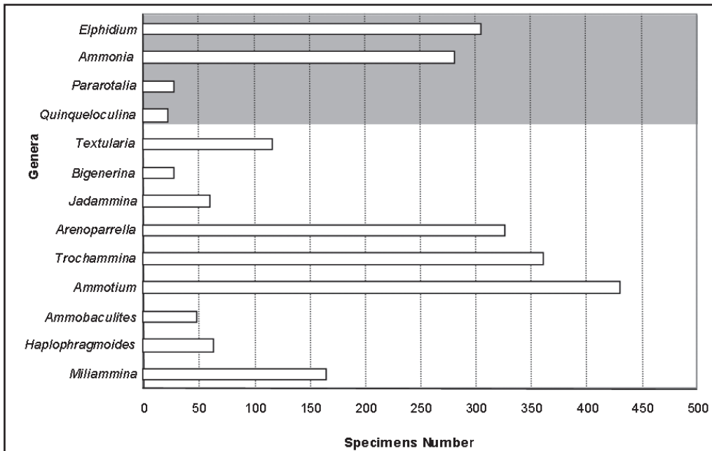
Figure 5 Representation of the foraminifera genera of the TCV2A core.
