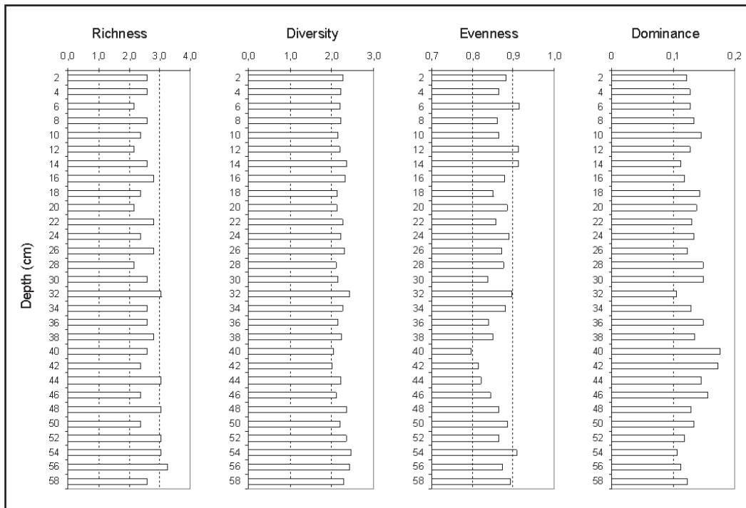
Figure 4 Vertical distribution of the richness, diversity, evenness and dominance indices along the TCV1A core.
