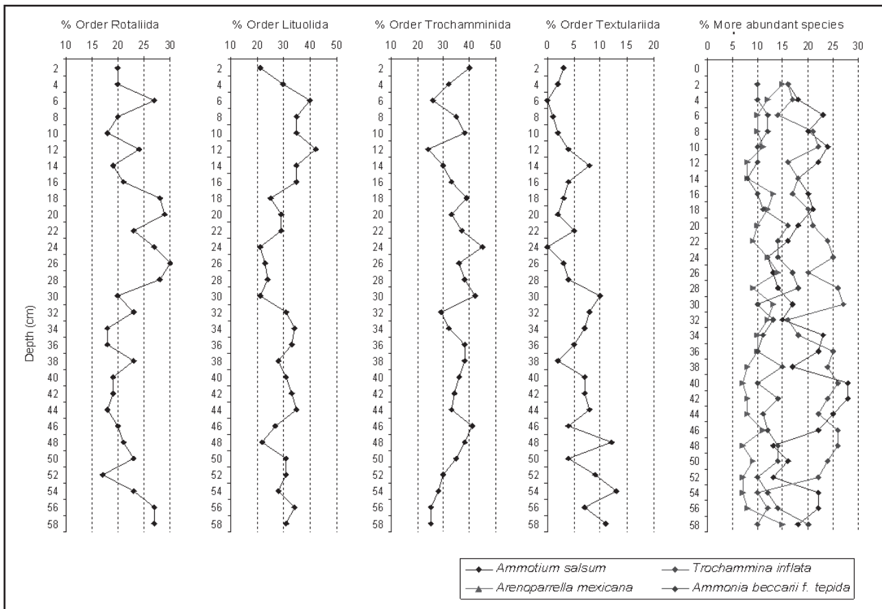
Figure 3 Vertical distribution of the identified orders and most abundant species along the TCVIA core.
