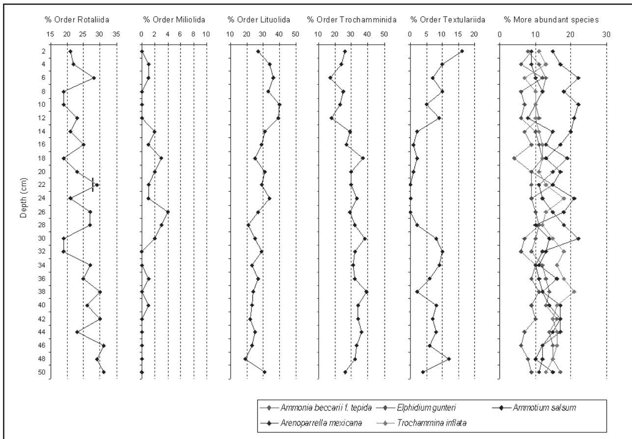
Figure 6 Vertical distribution of the identified orders e most abundant species along the TCV2A core.
